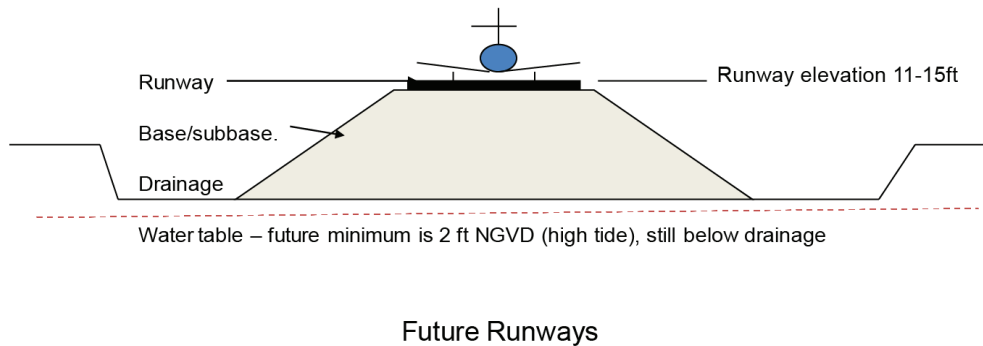
Figure 6.7 Sea level rise will threaten runways, but because runways are designed with elevation than roadways, runways will not be affected by inundation as early as are roadways or railroads.
