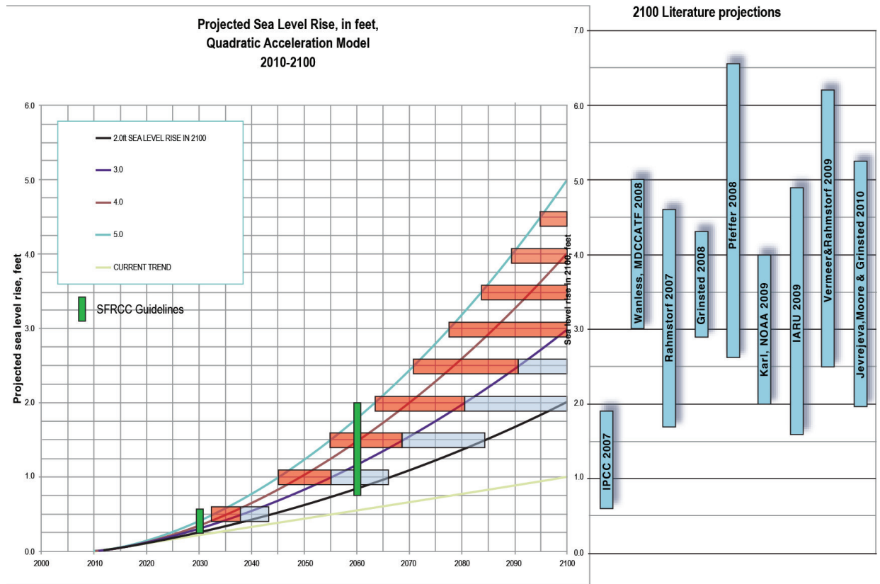
Figure 6.2 Prediction of Sea Level Rise, accoudnign for time and rise.
