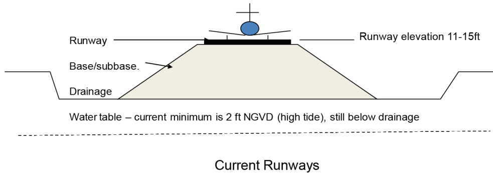
Figure 6.6 Figure 6.6 Airport runways are generally elevated.
