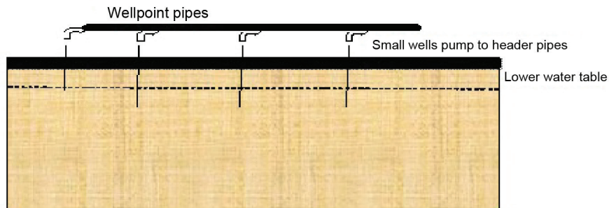
Figure 6.10 Wellpoints
