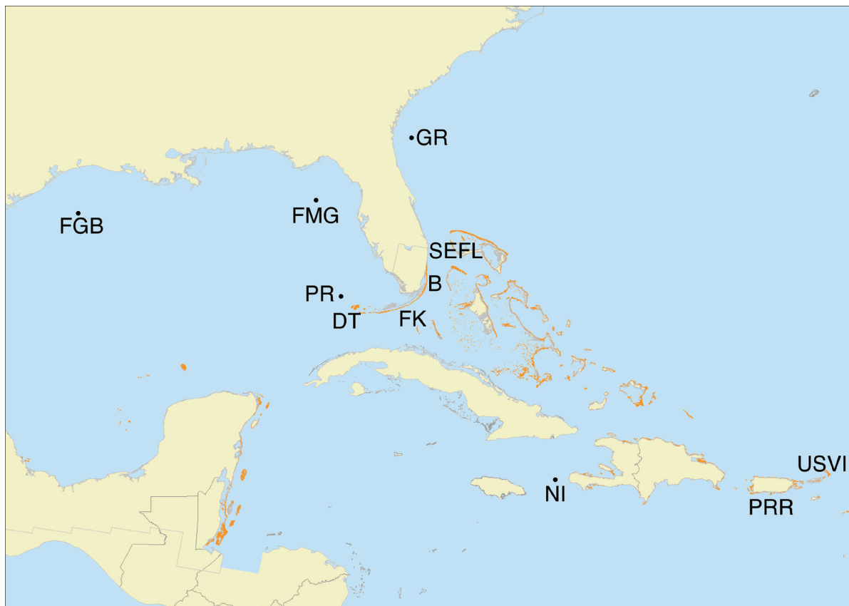
Figure 11.6 Location of coral reefs in the SE USA including Flower Garden Banks (FGB), Florida Middle Grounds (FMG), Pulley Ridge (PR), Dry Tortugas (DT), Florida Keys (FK), Biscayne (B), southeast Florida reefs (SEFL), Gray's Reef (GR), Navassa Island (NI), Puerto Rico (PRR), and US Virgin Islands (USVI). Orange areas are coral reefs from ReefBase ( http://reefgis.reefbase.org/ ).
