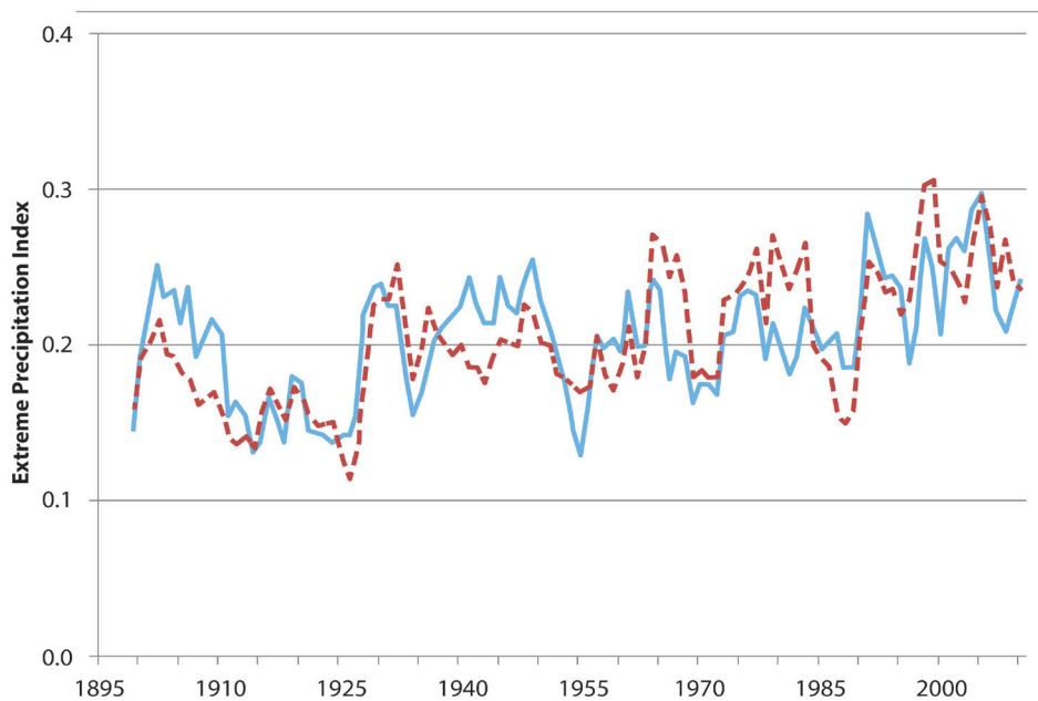
Figure 5.4 Trends in the extreme precipitation index for the southeastern USA. Red line is 1 day, 1 in 5-year event. Blue line is 5-day, 1 in 5-year event (Kunkel, pers. comm.).
